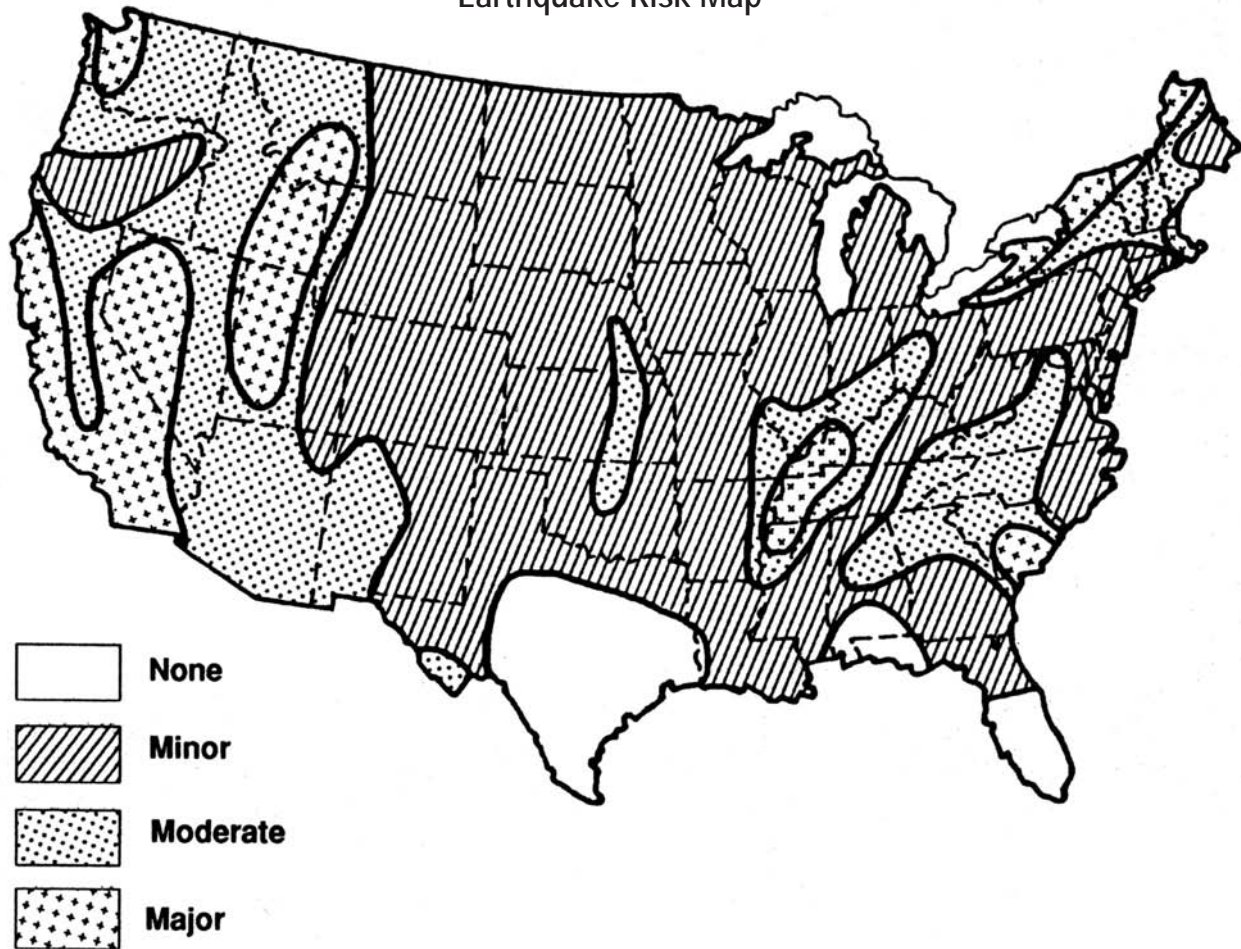
Earthquake Risk Map
